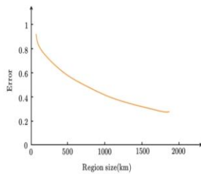
Figure 3: Decrease of forecast error for aggregated wind power prediction, based on data 40 wind farms in Germany (Holttinen et al., 2009)
